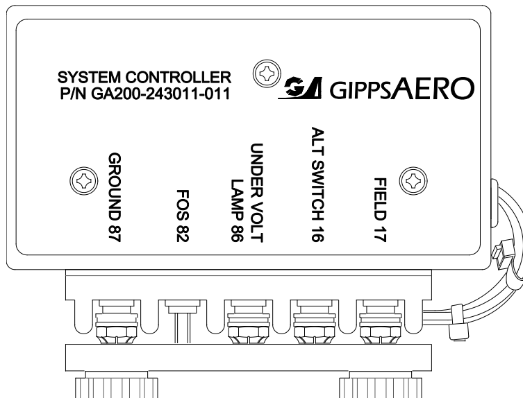
Figure 1 – System Controller GA200-243011-011.
